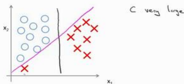
Large margin classifier in presence of outliers
